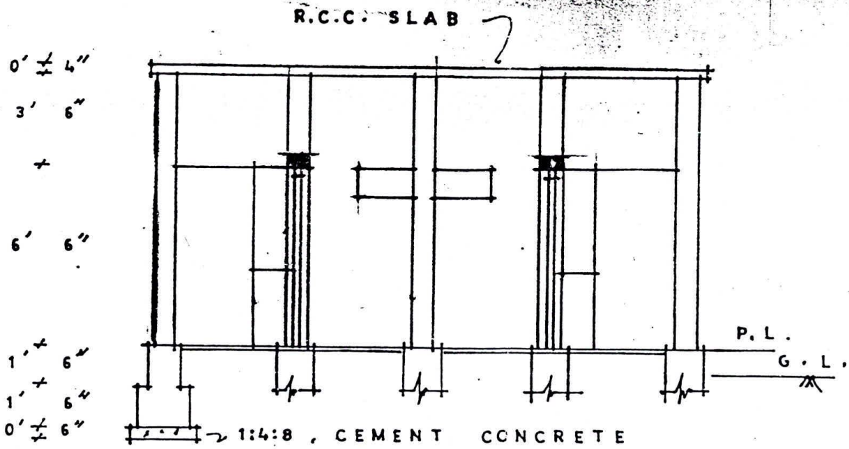
SECTION, A - B
