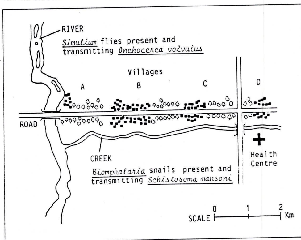
Figure 11.13. Local map showing the transmission sites of Onchocerca volvulus and Schistosoma mansoni close to villages A, B, C and D
