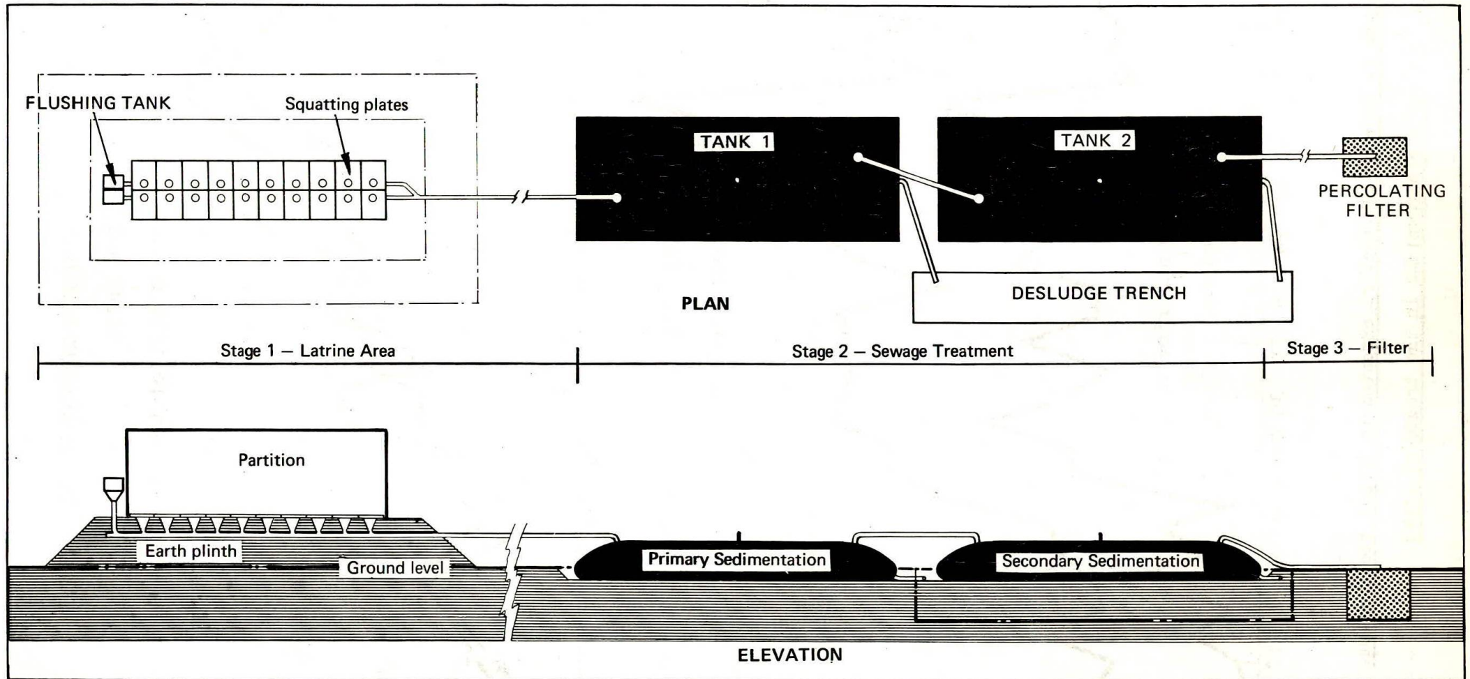
GENERAL LAYOUT OF SANITATION UNIT
